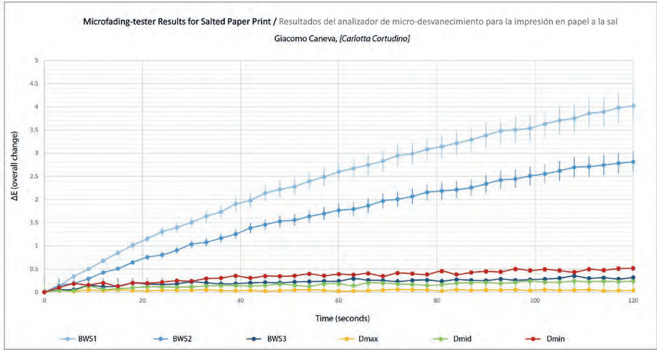
Figure 3 | Microfading-tester results for the salted paper print by Giacomo Caneva, [Carlotta Cortudino] (2005.100.57) (Fig. 2A). Three measurement sites in minimum (Dmin), medium (Dmid), and maximum (Dmax) image-density areas are juxtaposed against Blue Wool Standards 1-3 data gathered during the same session. All three test sites have a sensitivity equivalent to BWS 3, indicating that the photograph is less susceptible to light-induced color change.
