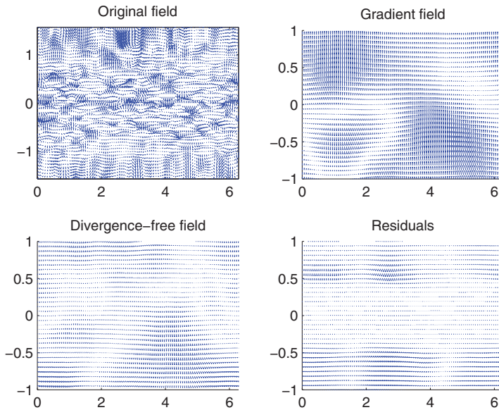
Figure 1. Original field, gradient field, divergence-free field and residual field.
